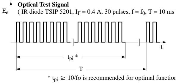
Figure 7. Output Function
